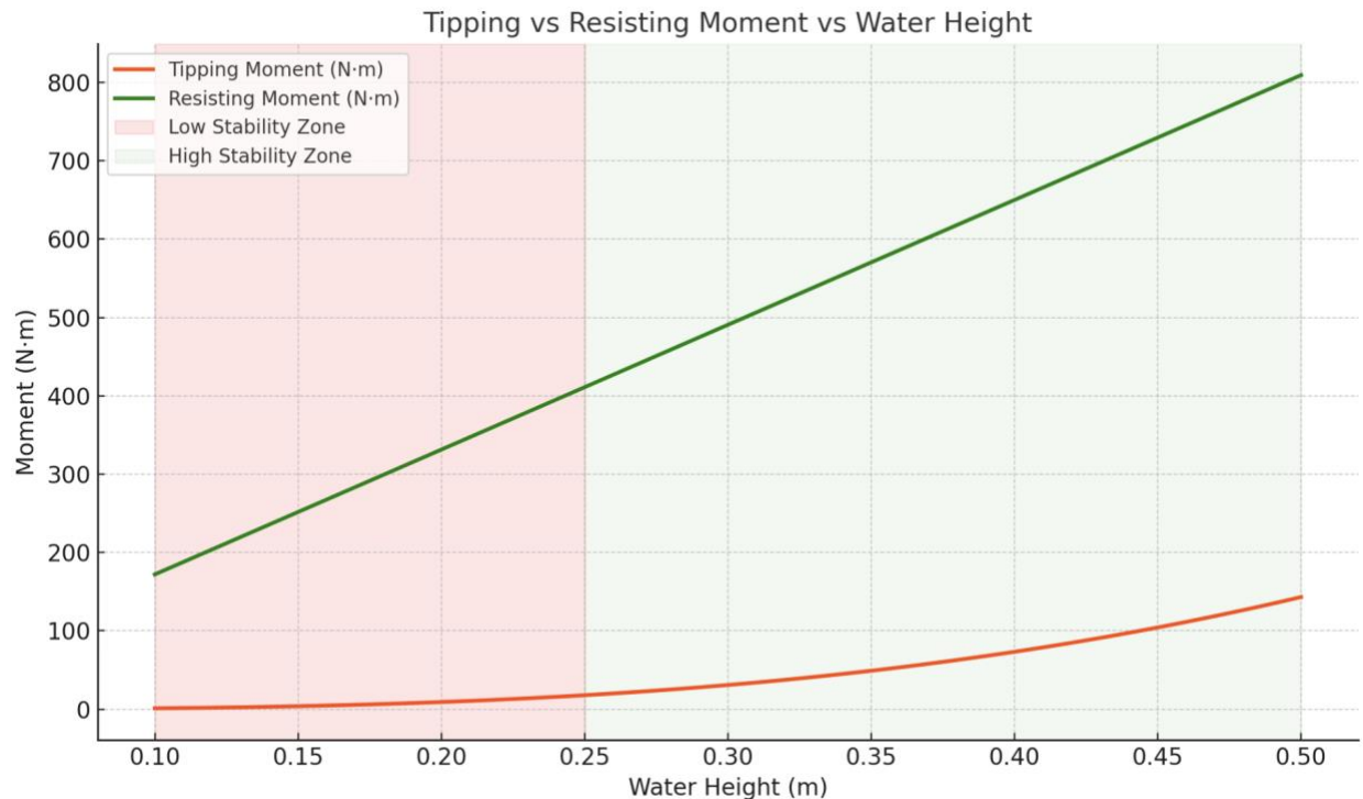
Graph 1: Tipping Moment vs Resisting Moment
