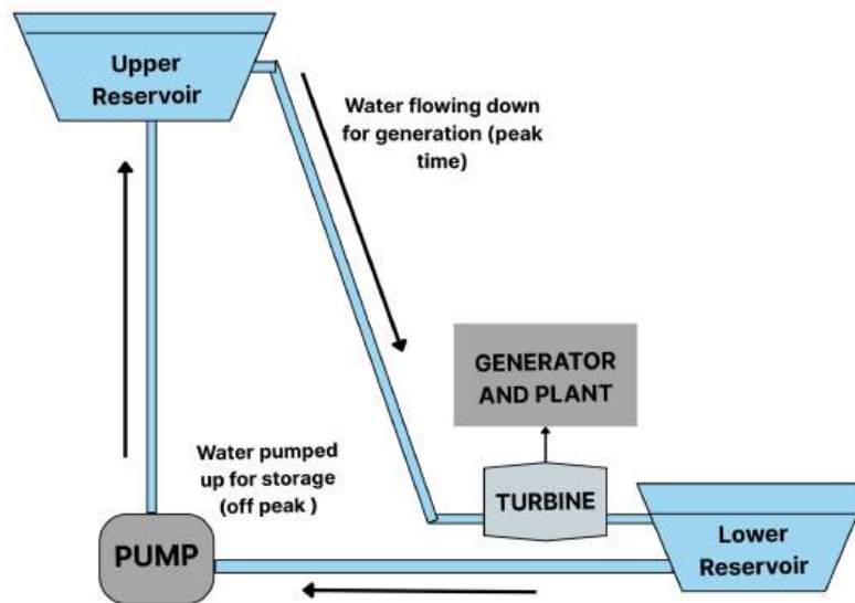
Figure 3: The diagram above displays the mechanics of a hydro-pump storage system.
