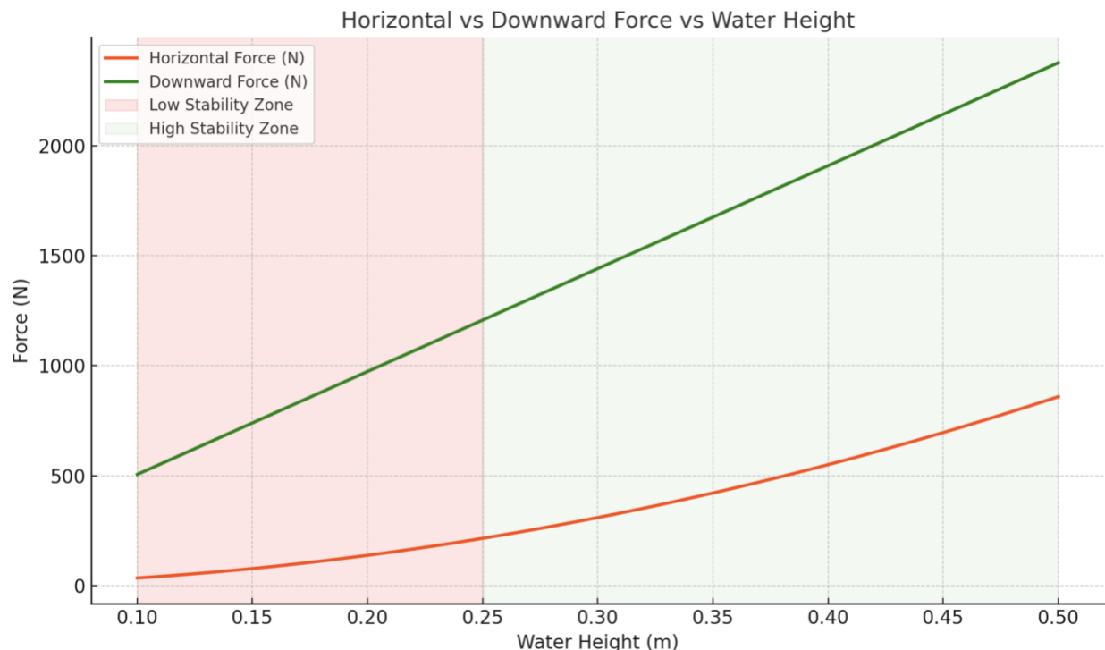
Graph 2: Horizontal Force vs Downward Force
