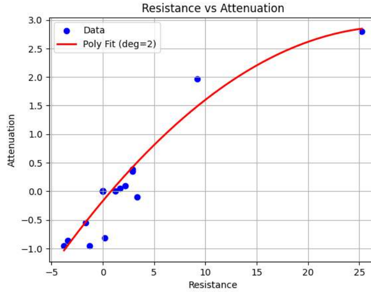
FIG. 3. Resistance vs Attenuation. Describes the relationship between the resistance of the coaxial cables used to transmit the microwave pulse to the qubit and the amount of lost signal in the microwave pulse. The resistance evolves through temperature, and the data was taken at 300 K, 77 K, and 13 K.
