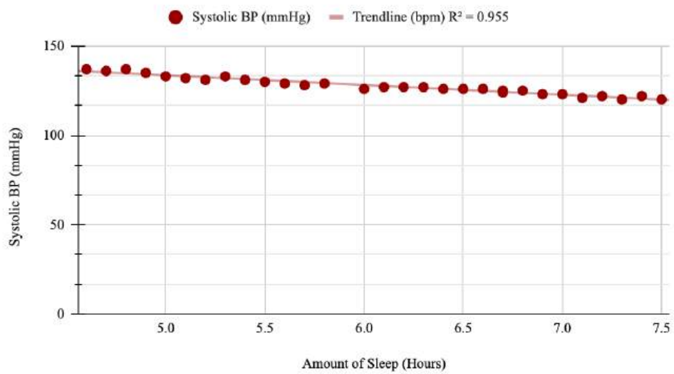
Figure 6. Scatter Plot of Sleep Hours vs Systolic BP
