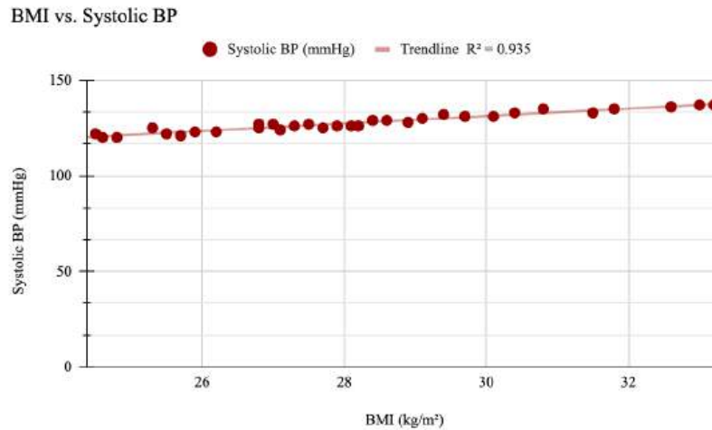
Figure 7. Scatter Plot of BMI vs Systolic BP
