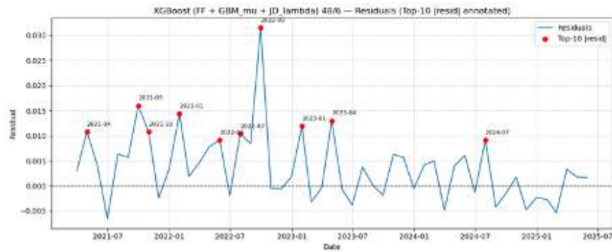
Figure 17: Residual Returns Over Time – Fama-French + GBM + JD + XGBoost Model
