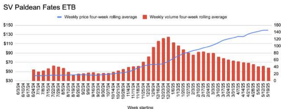
Fig 3: Scarlet & Violet Paldean Fates ETB graph. Correlation of averaged weekly price and volume sold: 11/4/24–12/30/24 (moderately strong positive correlation, R^2=0.79 ), 12/30/24–5/19/25 (strong negative correlation, R^2=0.95 ). Explanation of chosen dates and swap dates in the following section.
