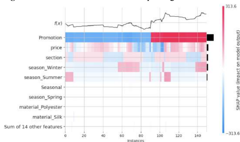
Figure 3. Feature contribution heatmap using SHAP values
