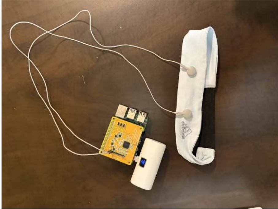
Fig 2: Headband and Electrodes attached to the PiEEG v2.1, Raspberry Pi 4, and portable ANKER charger.
