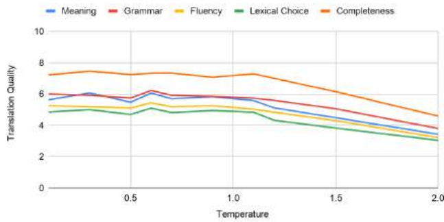
Figure 2.1: Illustration of a moderate sensitivity to temperature for Qwen 3 8B, EN→RU, Crime and Punishment, Chapter 2.
