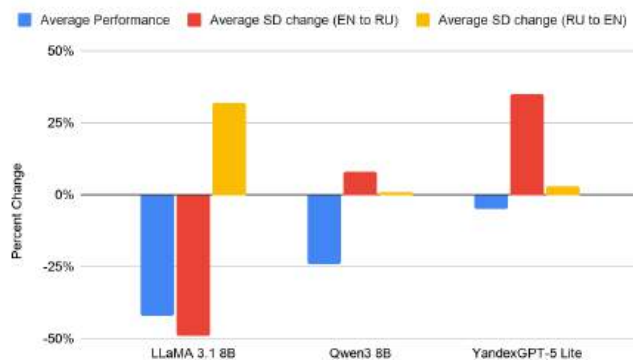
Figure 4.2: Illustrates performance and stability change across models.
