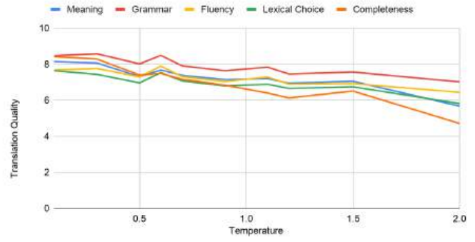
Figure 1.4: Illustration of the temperature changes' effect on performance for LLaMA 3.1 8B, RU→EN, RusLTC
