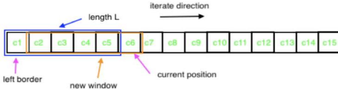
Figure 3 An Example of the Sliding Window Algorithm
