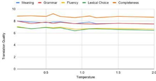
Figure 3.1: Illustration of a minimal sensitivity to temperature for YandexGPT 8B, EN→RU, Crime and Punishment, Chapter 2.
