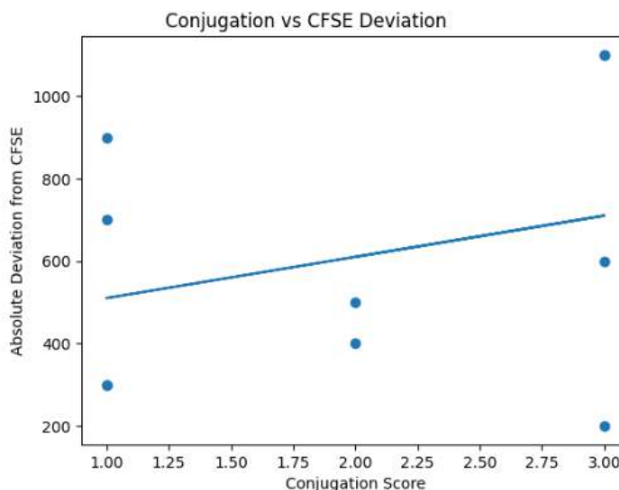
Figure 3. Ligand Conjugation Strength vs CFSE
