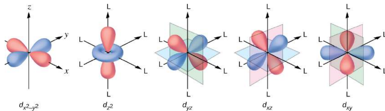
Figure 6. Geometric Visualizations of d-orbitals
