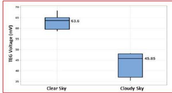
Figure 4. Box and whisker plots of thermo-electric generator (TEG) voltage output under clear sky and cloudy sky.
