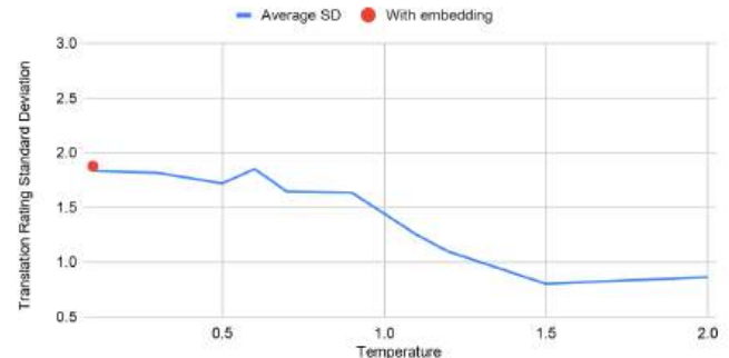
Figure 1.6: Relationship between temperature and the average SD across all evaluated translation categories for LLaMA 3.1 8B, EN→RU, RusLTC.
