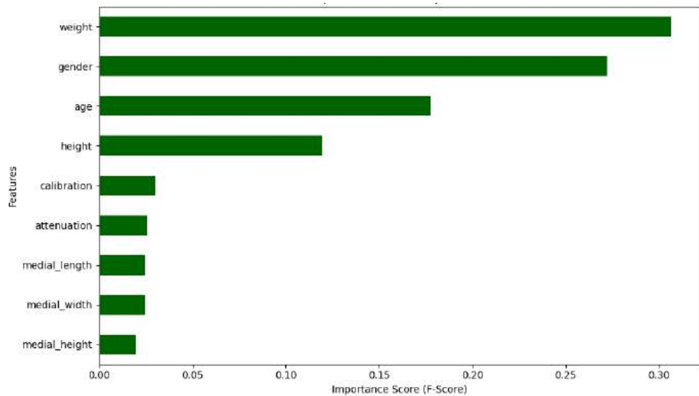
Figure 3: Relative importance scores (F-scores) for demographic, radiofrequency-based, and physical features used in the XGBoost model using the combined dataset. Demographic variables accounted for 87.6% of total feature importance, indicating they are the primary variables for classification, while radiofrequency-based features provide supplementary predictive signals.
