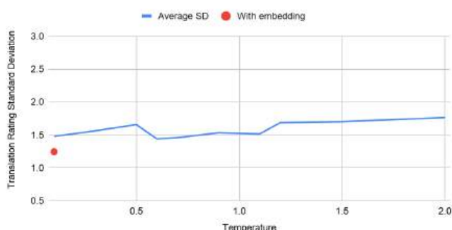
Figure 3.3: Presentation of the SD of translation scores for YandexGPT 8B, EN→RU, Crime and Punishment, Chapter 2.
