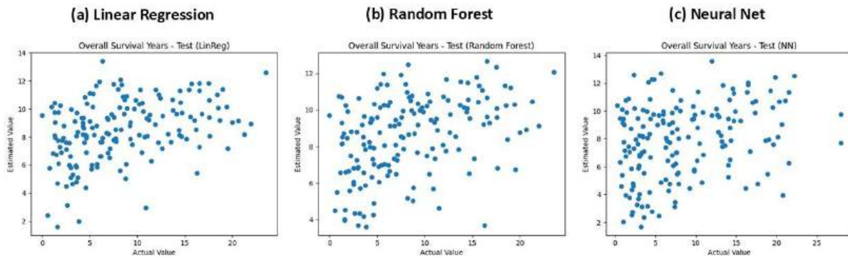
Figure 2. Comparison of actual versus estimated actual survival years for models run on the test set. (a) Linear regression comparison. (b) Random forest comparison. (c) Neural network comparison.
