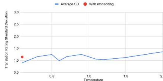
Figure 3.4: Presentation of the SD of translation scores for YandexGPT 8B, EN→RU, RusLTC.
