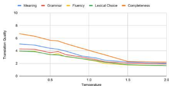
Figure 1.2: Illustration of relation between the temperature and category-based scores for LLaMA 3.1 8B, EN→RU, RusLTC
