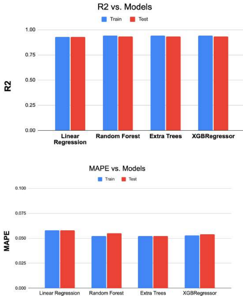
Figure 1. Train and test (top) R^2 and (bottom) MAPE of the models
