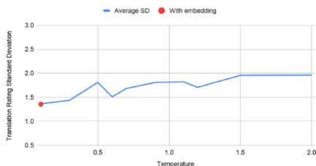
Figure 1.8: Illustrates the increase of the SD as temperature rises for LLaMA 3.1 8B, RU→EN, RusLTC.
