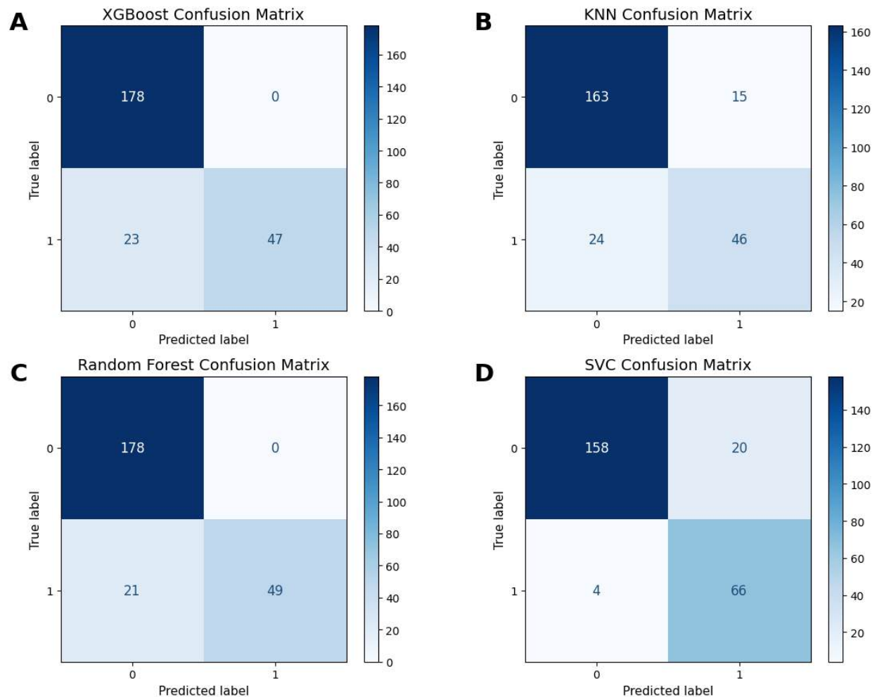
Figure 2: Confusion matrices for XGBoost (A), KNN (B), Random Forest (C), and SVC (D) models using the combined dataset on the independent test set. SVC indicated the fewest false negatives but also the most false positives, which indicates that specificity may be sacrificed when sensitivity is improved.
