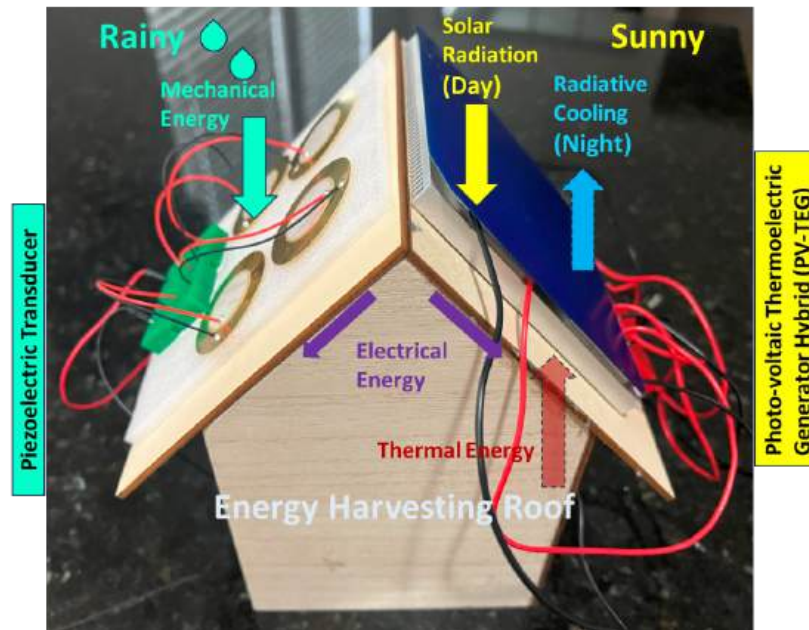
Figure 1. Energy harvesting roof consisting of a Piezoelectric roof and PV-TEG roof PV-TEG Hybrid Roof
