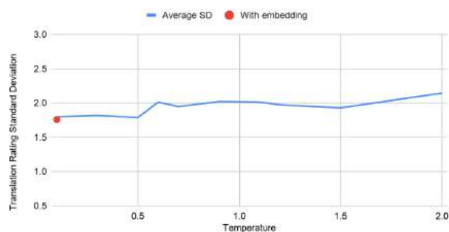
Figure 1.7: Illustrates increase of the SD as temperature rises for LLaMA 3.1 8B, RU→EN, Crime and Punishment, Chapter 2.
