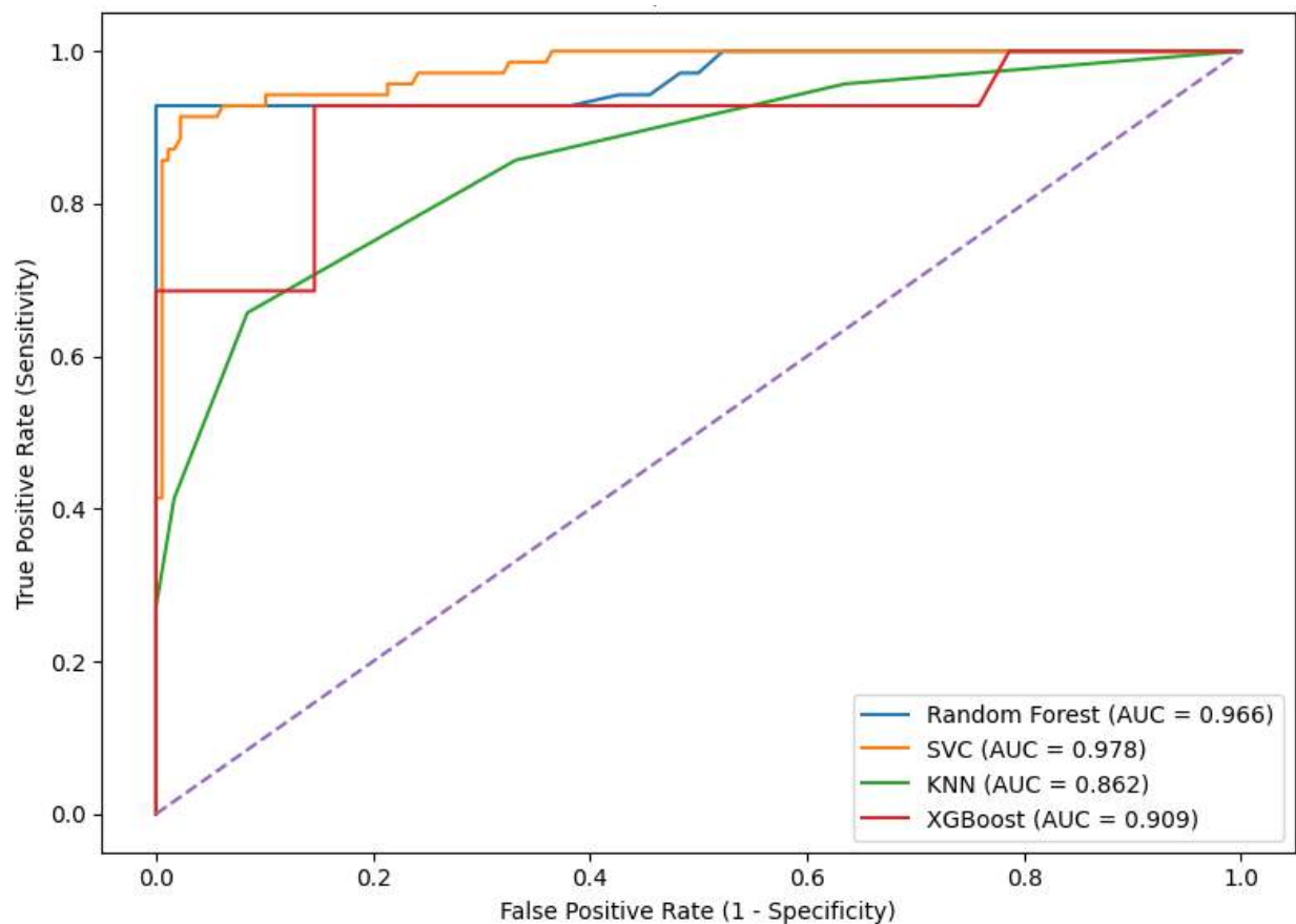
Figure 1: ROC curves for the Random Forest, SVC, KNN, and XGBoost classification models with the combined dataset (true positive rate vs. false positive rate). SVC and Random Forest had the strongest discrimination ability, meaning they can most reliably separate osteoporotic from non-osteoporotic individuals for all classification thresholds.
