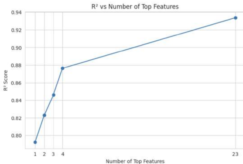
Figure 4. Effect of top features on model performance ( R^2 )
