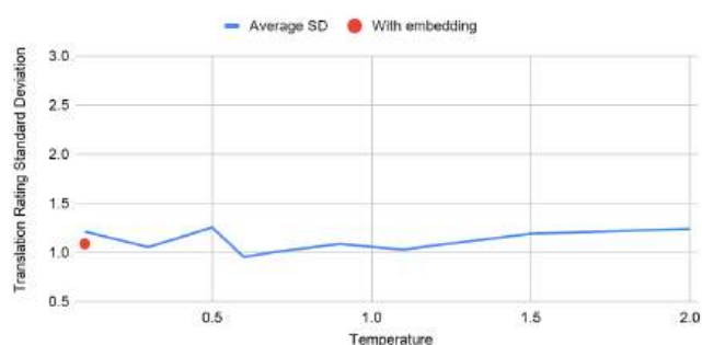
Figure 2.4: Presentation of the SD of translation scores for Qwen 3 8B, RU→EN, RusLTC.
