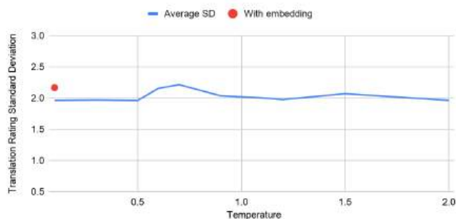
Figure 2.3: Presentation of the SD of translation scores for Qwen 3 8B, EN→RU, Crime and Punishment, Chapter 2.
