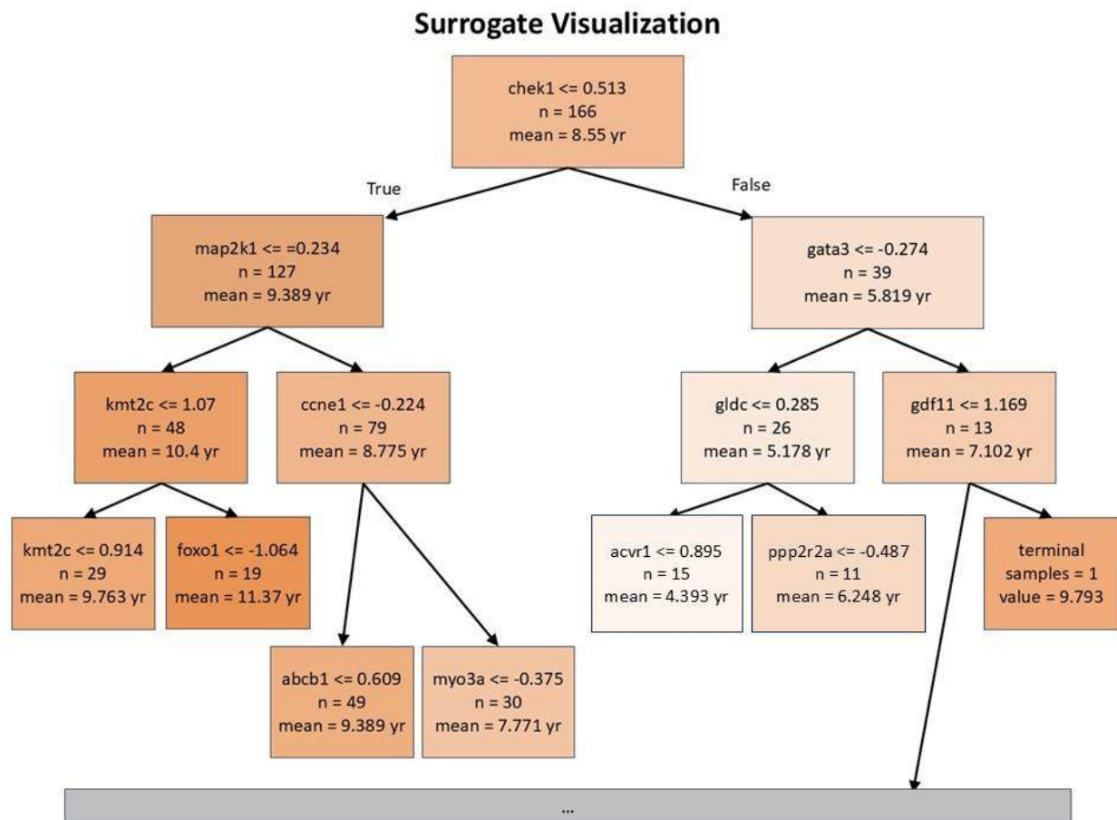
Figure 4. Surrogate tree visualization. Displays simplified version of the decision splits made by the model at the first three layers, deeper branches omitted for visibility.
