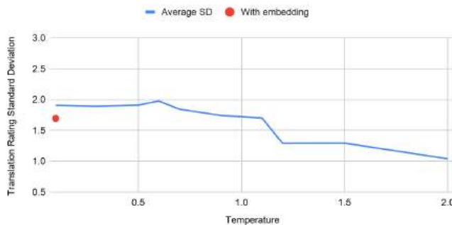
Figure 1.5: Relationship between temperature and the average SD across all evaluated translation categories for LLaMA 3.1 8B, EN→RU, Crime and Punishment, Chapter 2.
