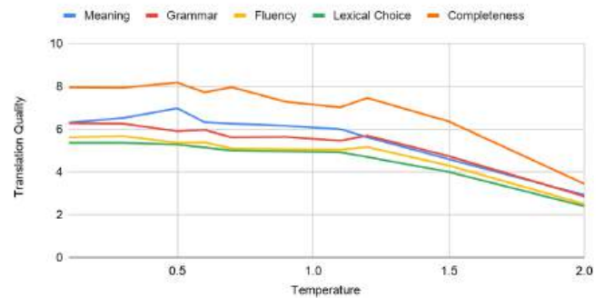
Figure 2.2: Illustration of a moderate sensitivity to temperature for Qwen 3 8B, EN→RU, RusLTC.
