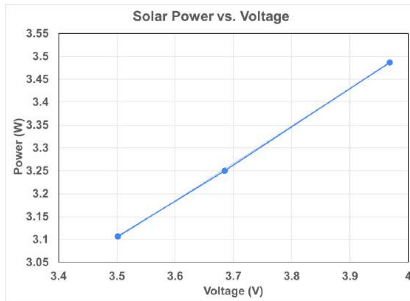
Figure 3. Line plot of mean solar power generated vs. mean voltage using solar cell
