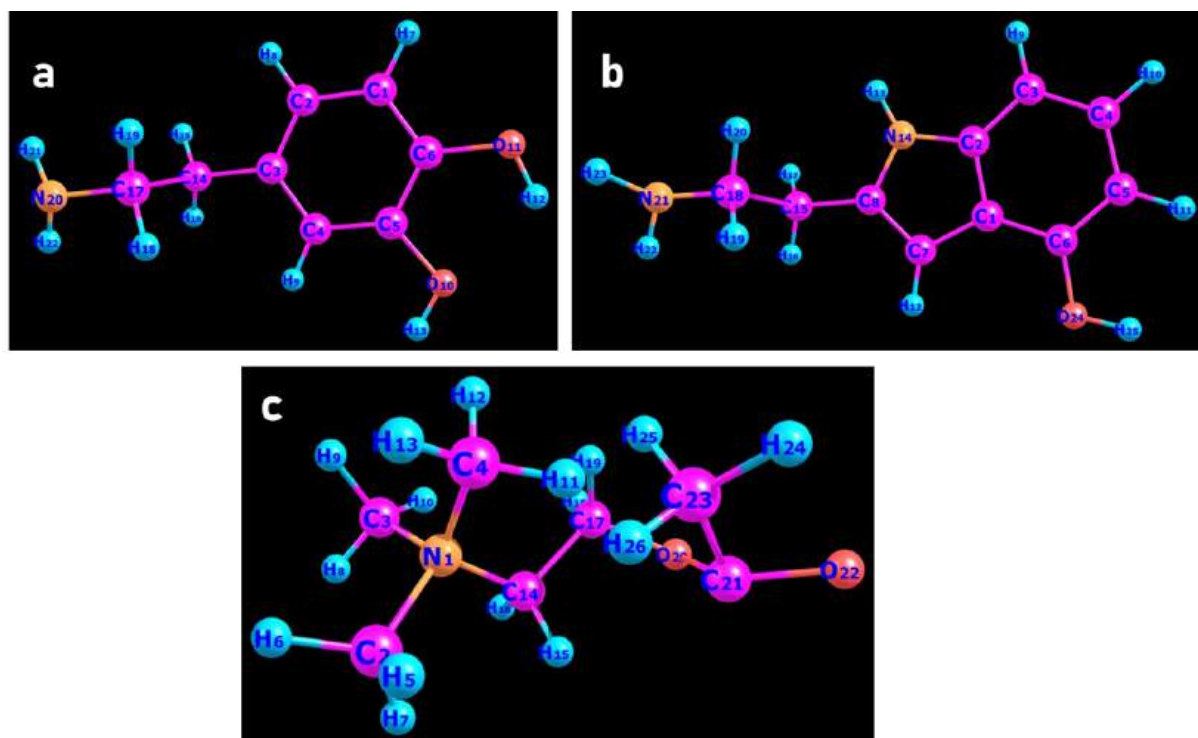
Figure 1. Optimised geometries of (a) Dopamine, (b) Serotonin, and (c) Acetylcholine in gas phase; Method/Basis set: B3LYP/6-31G
