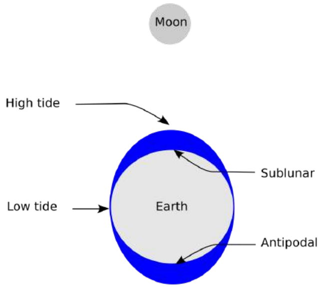
Fig 1: The Moon's gravity causes the ocean to bulge on both the side facing the Moon and the opposite side of the Earth. As a result, high tide occurs in these two regions, while low tide occurs in the regions between them.
