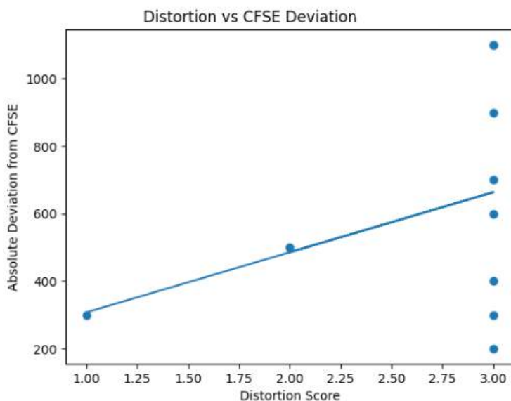
Figure 2. Ligand Distortion Strength vs CFSE
