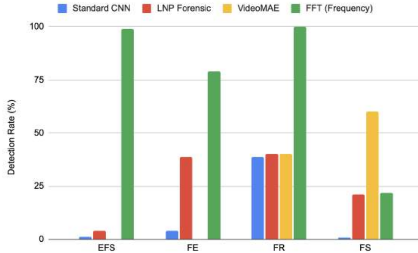
Fig 3: Comparative deepfake detection rates by tool and manipulation category
