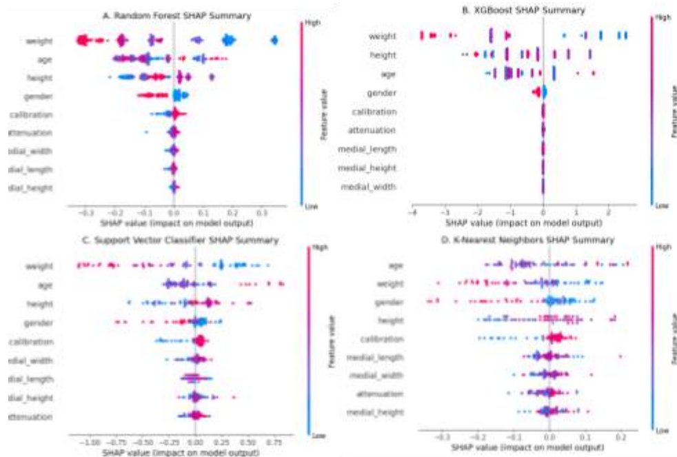
Figure 4: SHAP summary plots for the Random Forest (A), XGBoost (B), Support Vector Classifier (C), and K-Nearest Neighbors (D) models. Each plot shows the direction and magnitude of feature contributions for individual predictions. Importantly, the influence of radiofrequency-derived features varied by model type.
