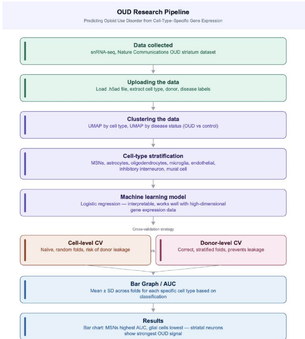
Figure 1: Pipeline for predicting OUD from cell-type gene expression in human dorsal striatum
