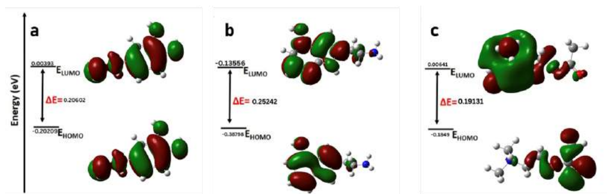
Figure 2. HOMO-LUMO diagrams of the optimised geometries of (a) Dopamine, (b) Serotonin, and (c) Acetylcholine in the gas phase. Method/Basis set: B3LYP/6-31G
