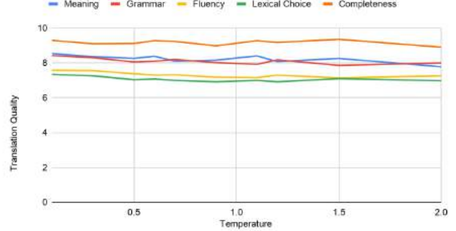
Figure 3.2: Illustration of a minimal sensitivity to temperature for YandexGPT 8B, EN→RU, RusLTC.
