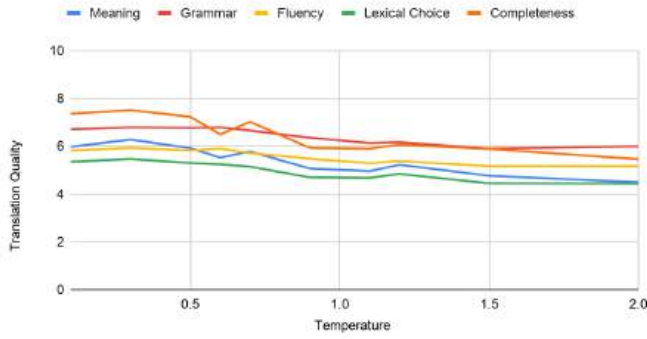
Figure 1.3: Illustration of the temperature changes' effect on performance for LLaMA 3.1 8B, RU→EN, Crime and Punishment, Chapter 2.
