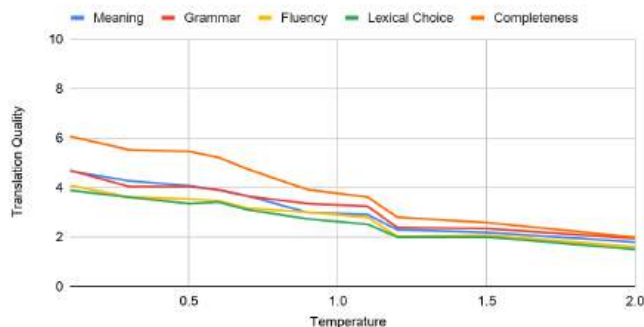
Figure 1.1: Illustration of relation between the temperature and category-based scores for LLaMA 3.1 8B, EN→RU, Crime and Punishment, Chapter 2.
