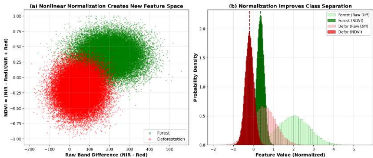
Figure 4.X: Feature Space Geometry
