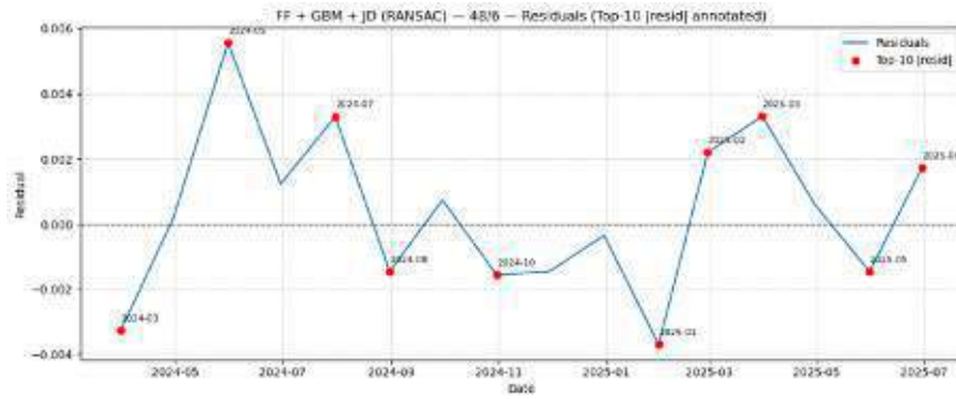
Figure 13: Residual Returns Over Time – Fama-French + GBM + JD + RANSAC Model
