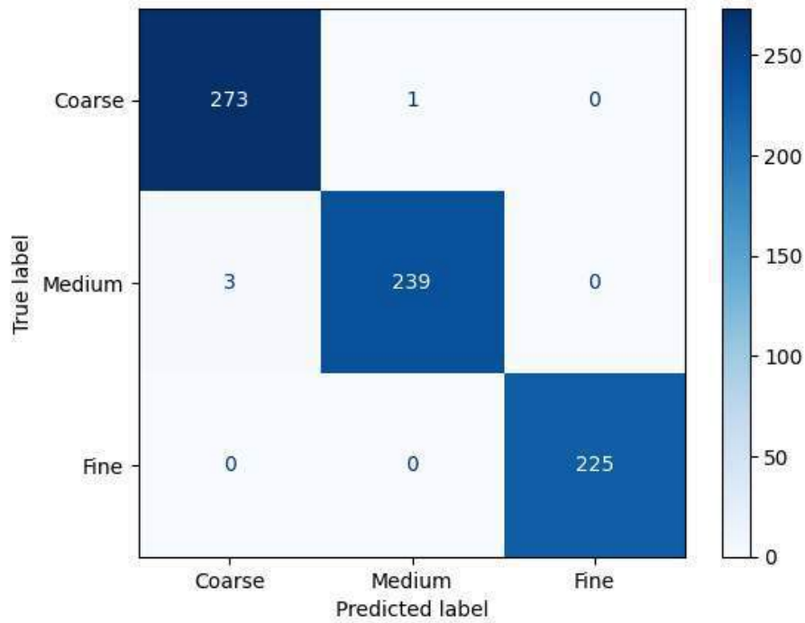
Figure 3. Confusion Matrix for the SoilNet prediction
