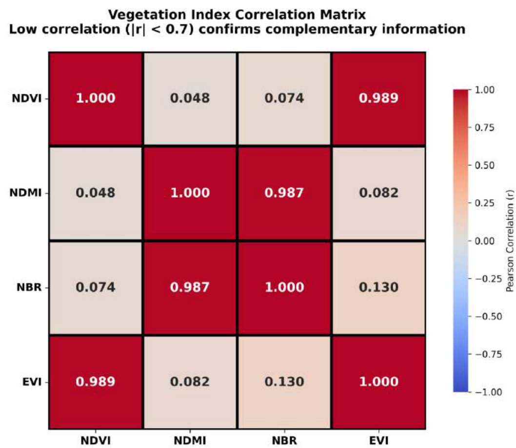
Figure 4.Y: Index Decorrelation Matrix
