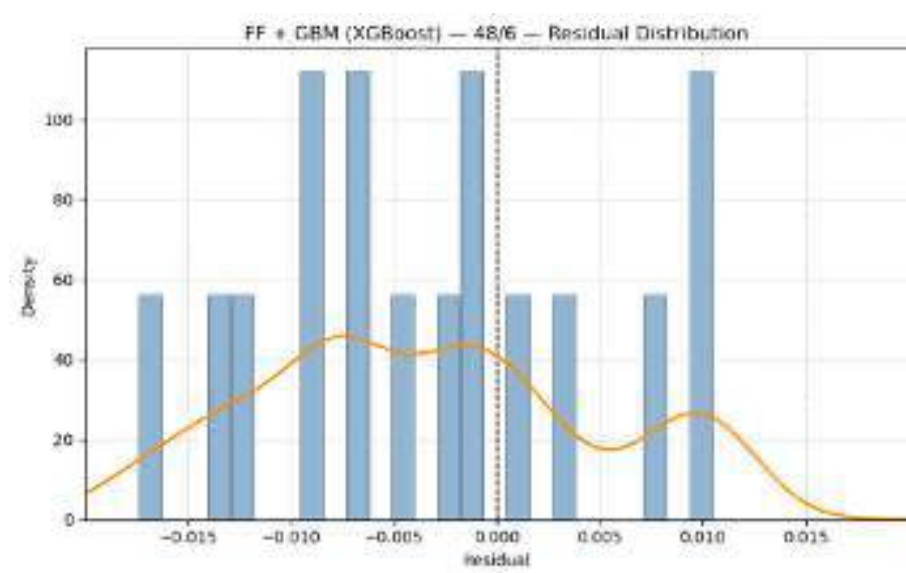
Figure 12: Residual Return Distribution – Fama-French + GBM + XGBoost Model
