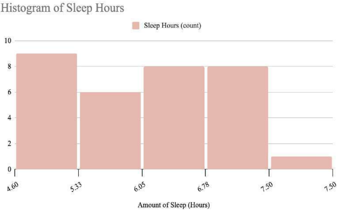
Figure 7. Histogram of Sleep Hours
